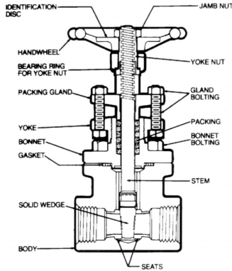
Gate Valve
