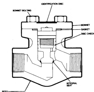
Check Valve
