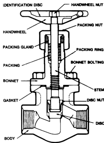
Globe Valve
